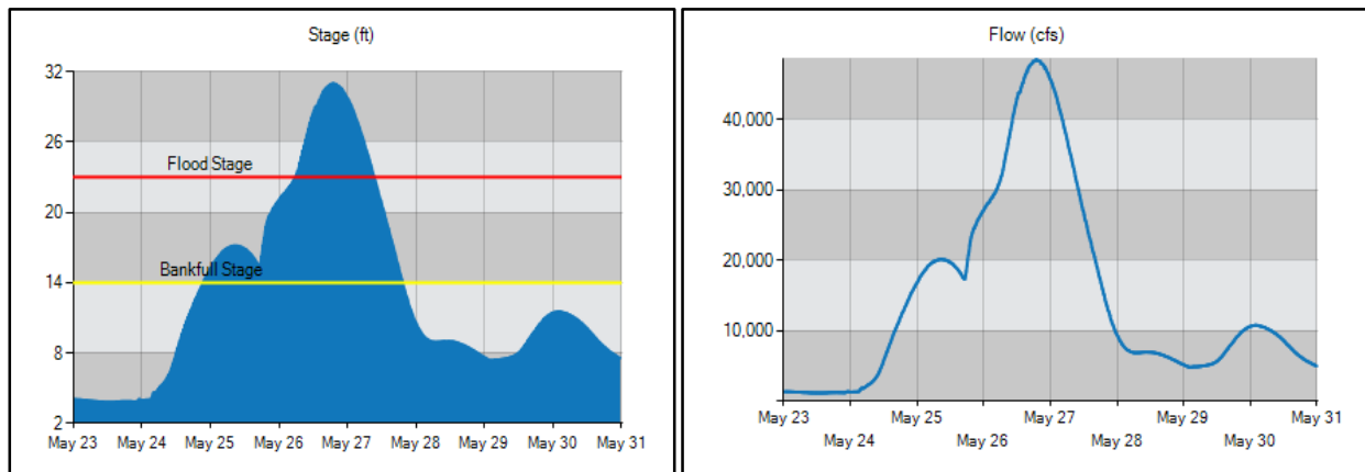
Figure 9-7. Colorado River at Bastrop Water Surface Elevation and Flow During the May 2015 Precipitation Event
