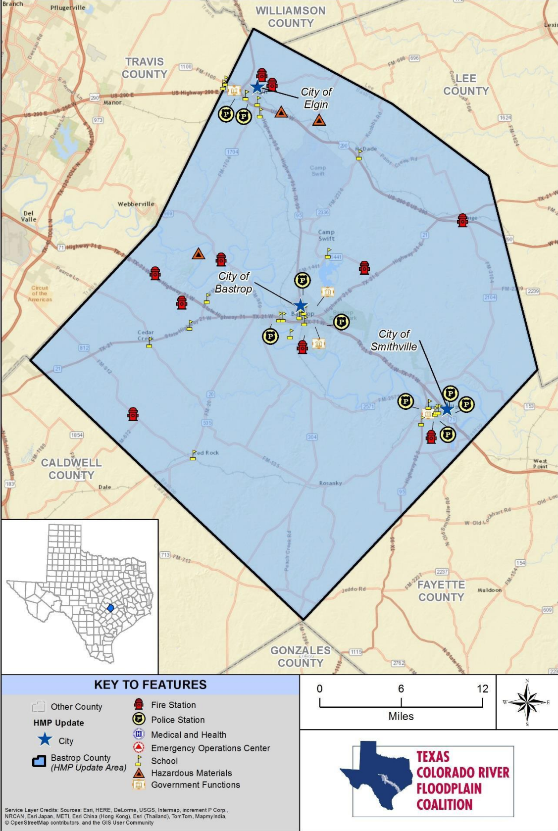
Figure 6-8. Critical Facilities in Bastrop County
