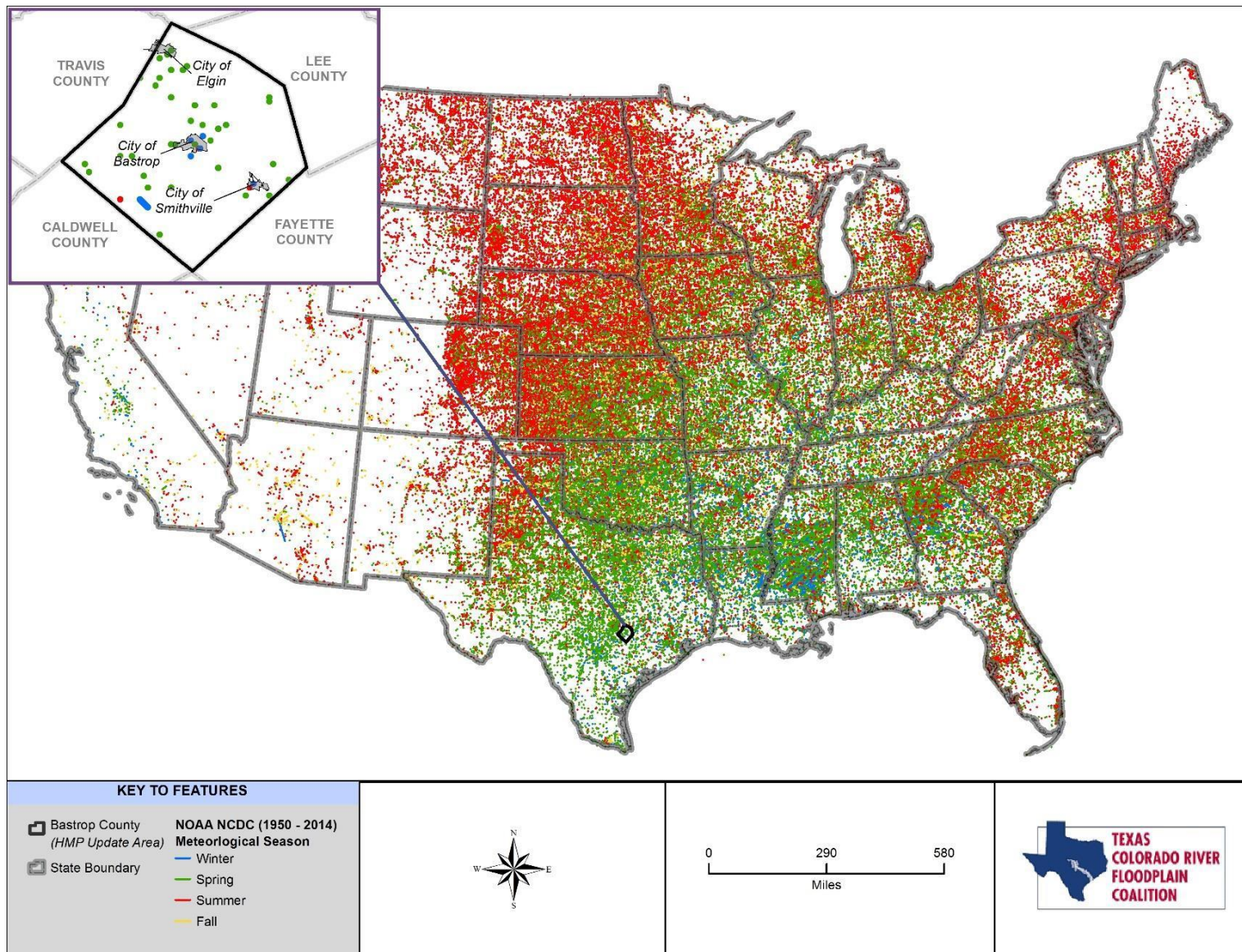
Figure 14-3. National Hail Paths
