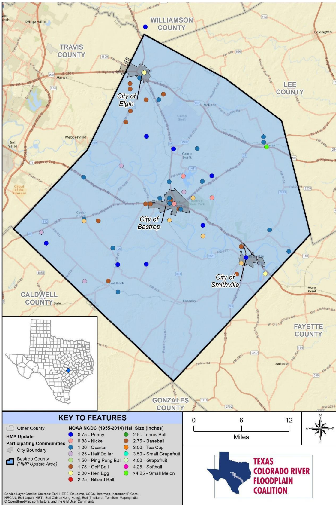
Figure 14-11. Hail Events in Bastrop County (1955-2014)
