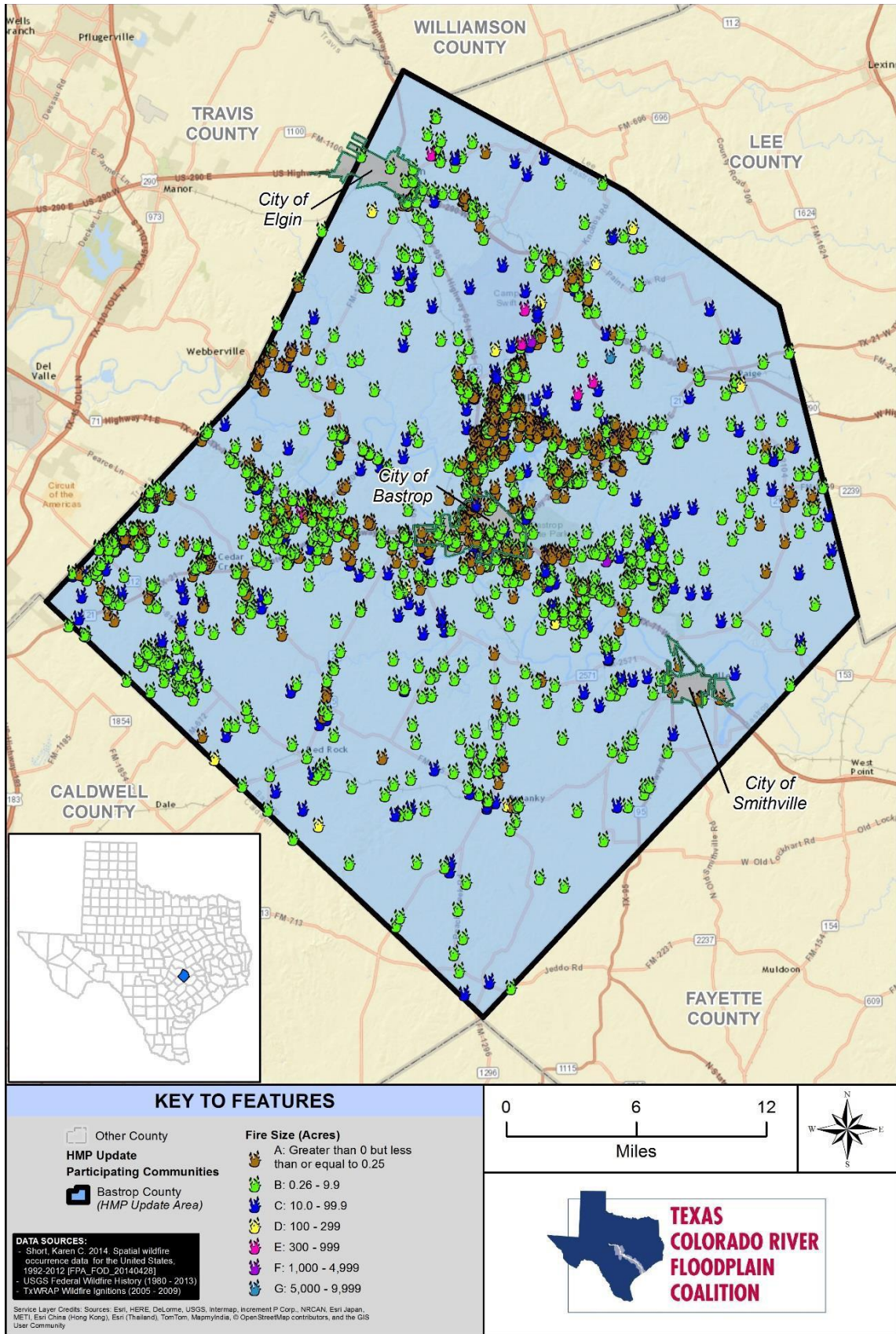
Figure 16-2. Wildfires in Bastrop County (1980-2014)
