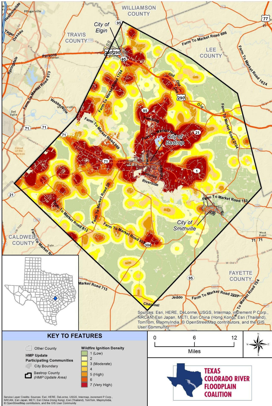
Figure 16-11. Bastrop County Wildfire and Participating Communities Ignitions Distribution
