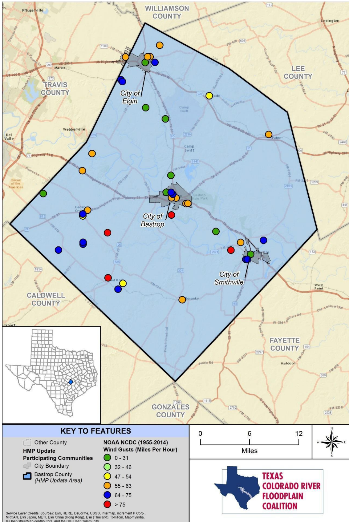
Figure 14-12. Damaging Wind Events in Bastrop County (1955-2014)
