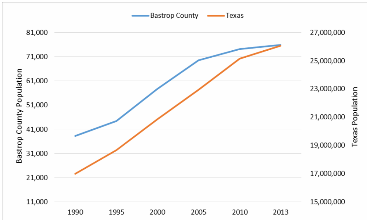
Figure 6-16. State of Texas and Bastrop County Population Growth
