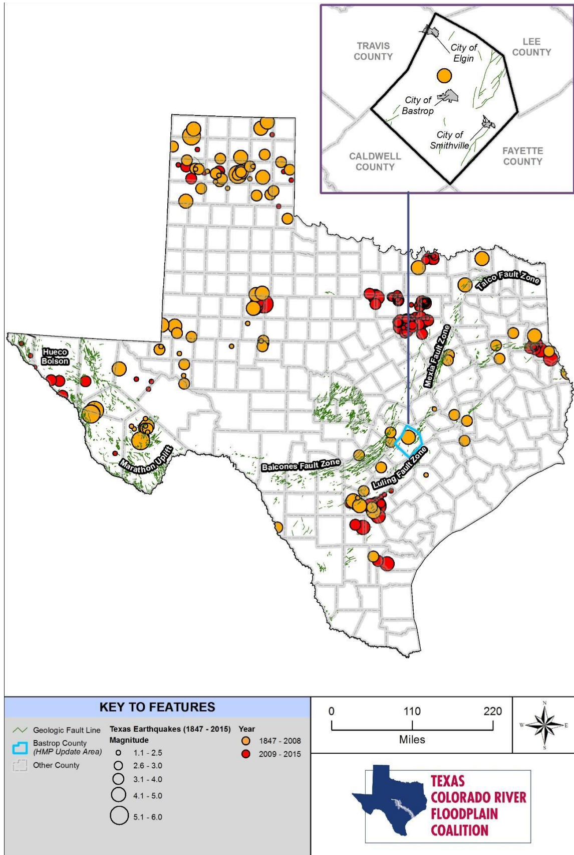
Figure 11-1. Texas Earthquakes (1847-2015)
