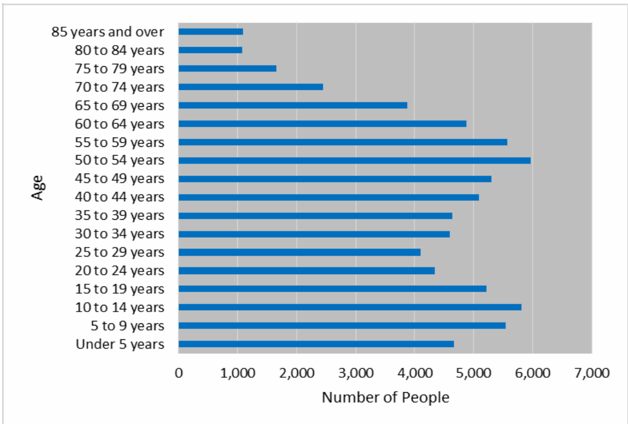
Figure 6-17. Bastrop County Age Distribution
