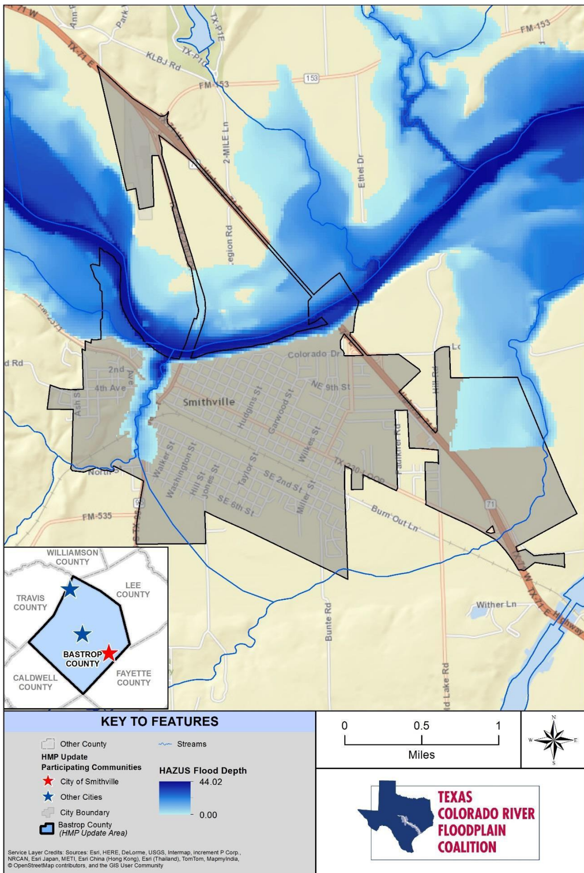
Figure 12-13. Flood Depths in the City of Smithville
