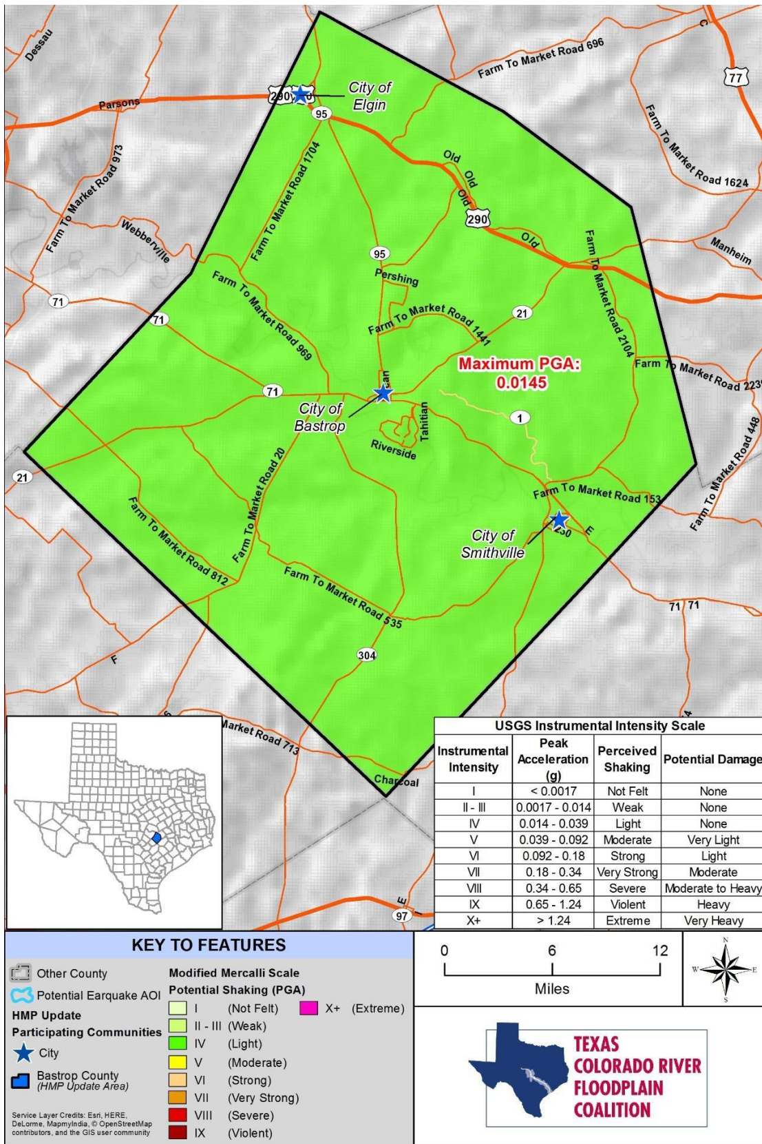
Figure 11-4. 500-Year Probability Event in Bastrop County
