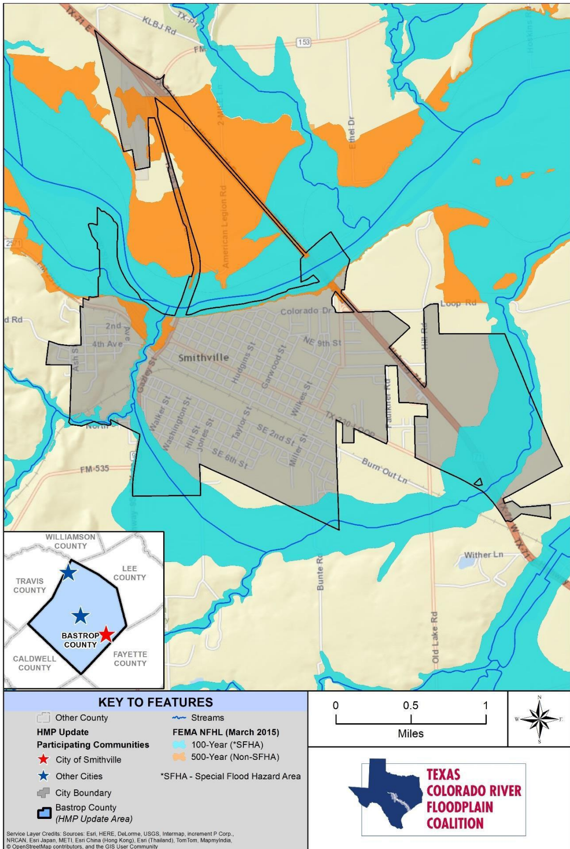
Figure 12-9. Special Flood Hazard Areas in the City of Smithville
