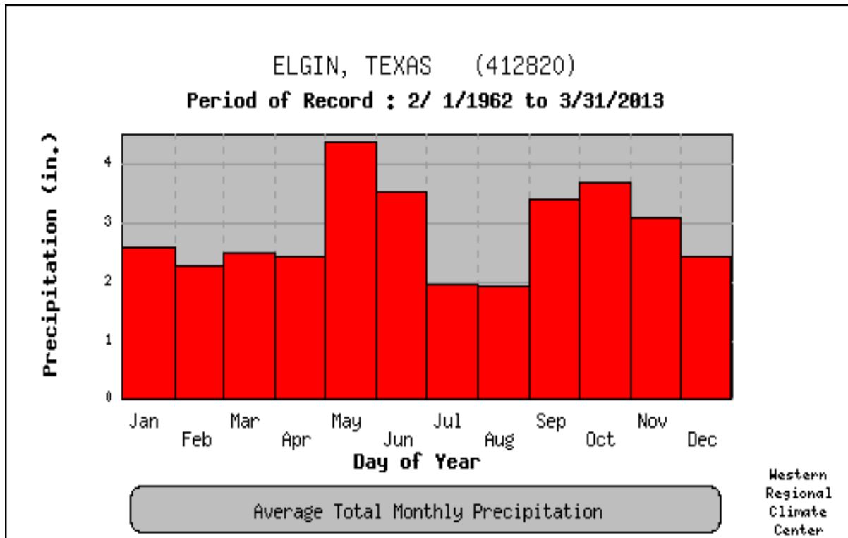
Figure 6-5. Average Monthly Precipitation (1962-2013)
