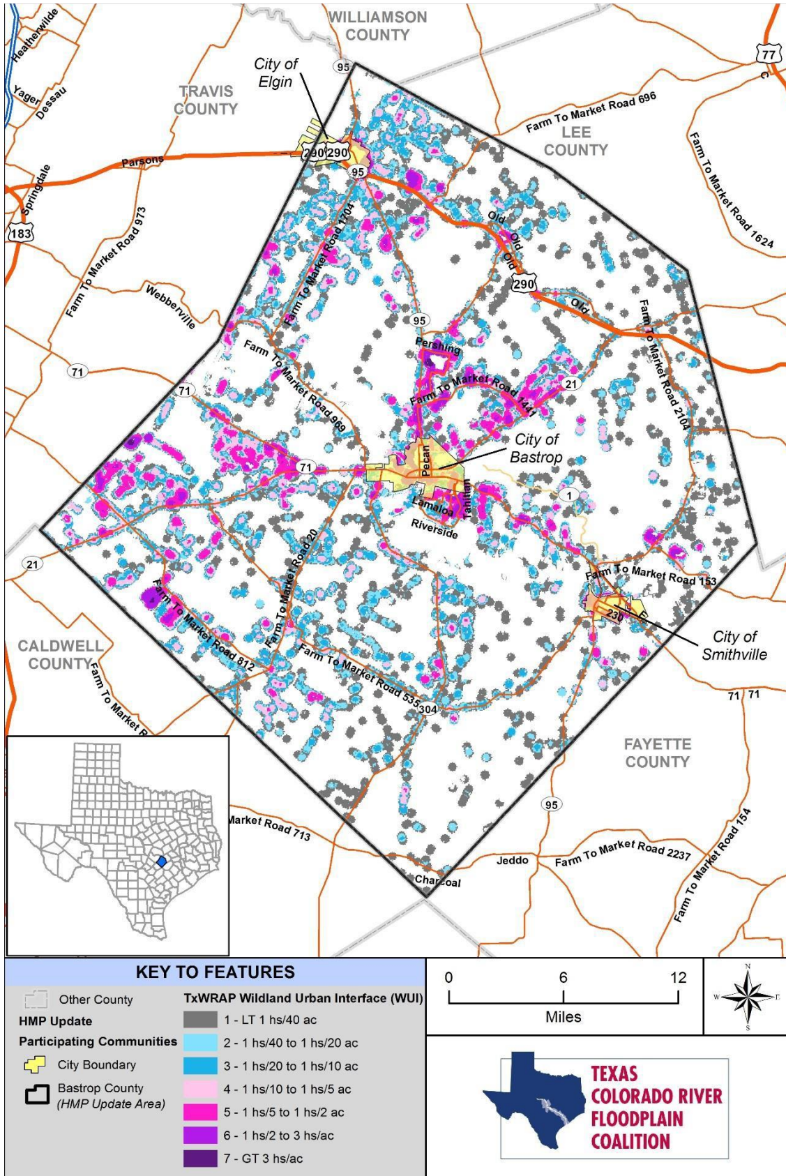
Figure 16-12. Bastrop County and Participating Communities Wildland Urban Interface
