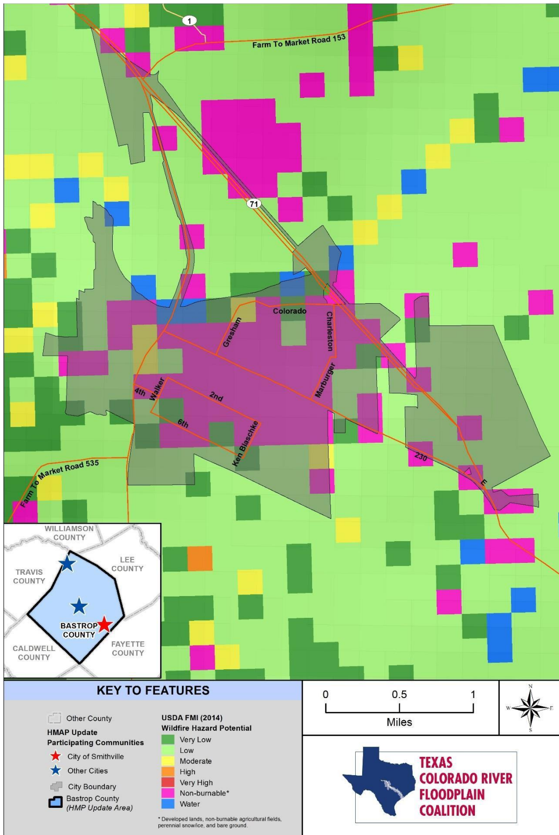
Figure 16-19. City of Smithville Wildfire Hazard Potential
