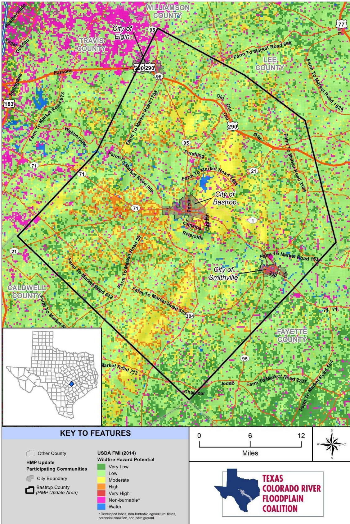
Figure 16-16. Bastrop County Wildfire Hazard Potential
