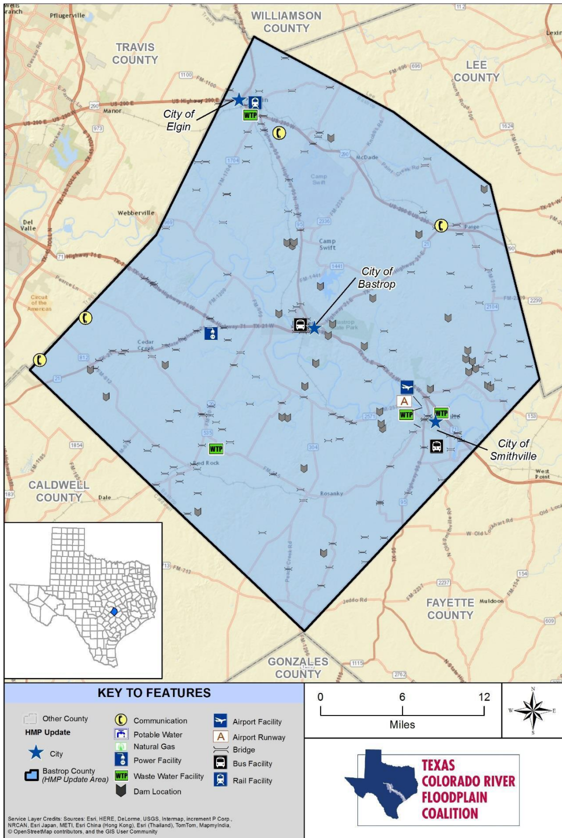
Figure 6-9. Critical Infrastructure in Bastrop County
