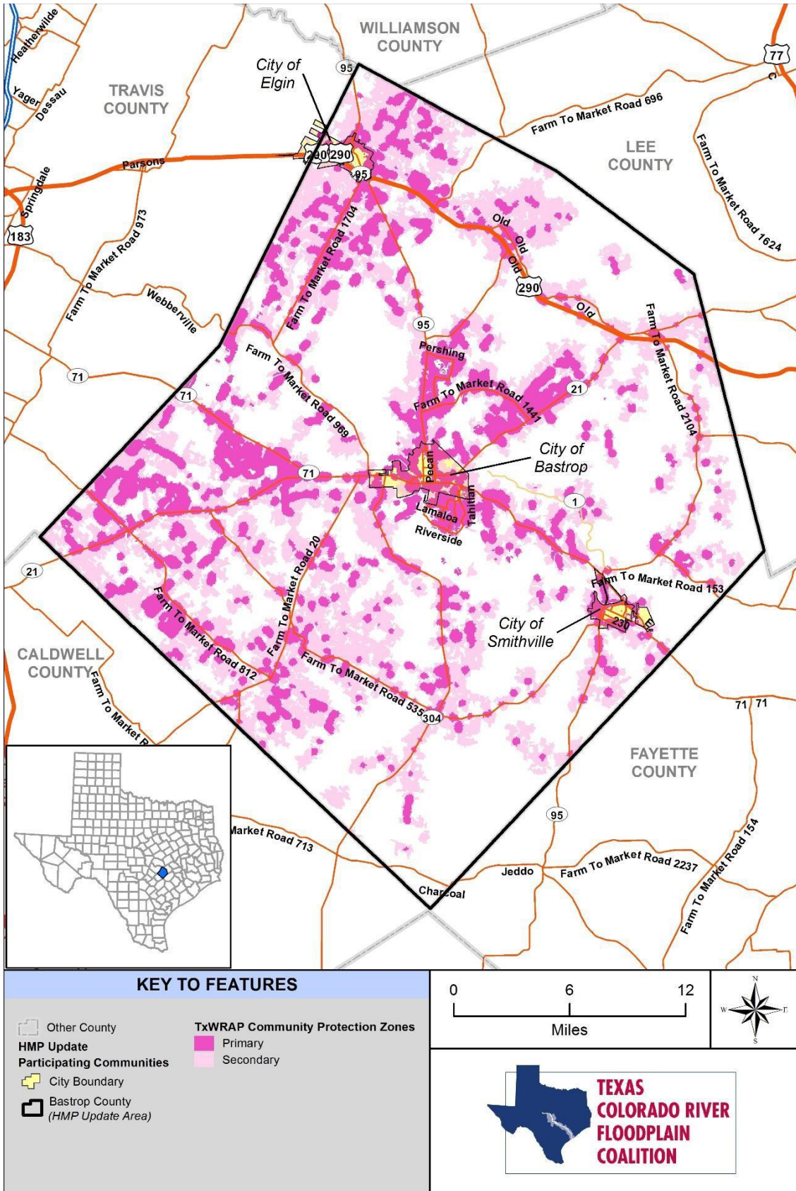
Figure 16-15. Bastrop County and Participating Communities Wildfire Community Protection Zones
