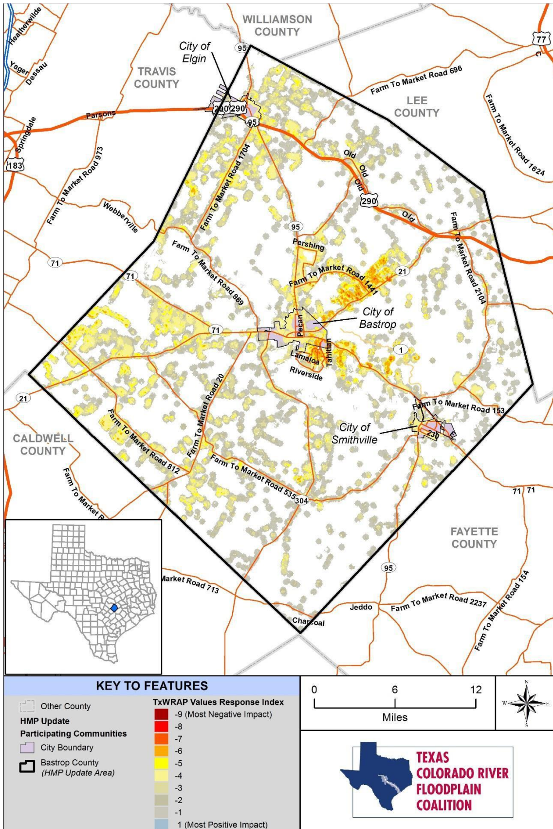
Figure 16-14. Bastrop County and Participating Communities Wildfire Values Response Index
