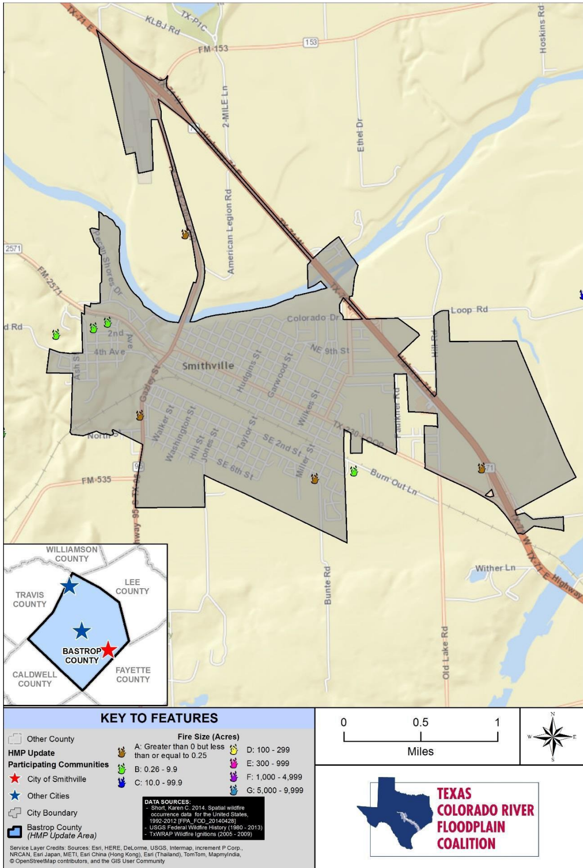
Figure 16-5. Wildfires in the City of Smithville (1980-2014)
