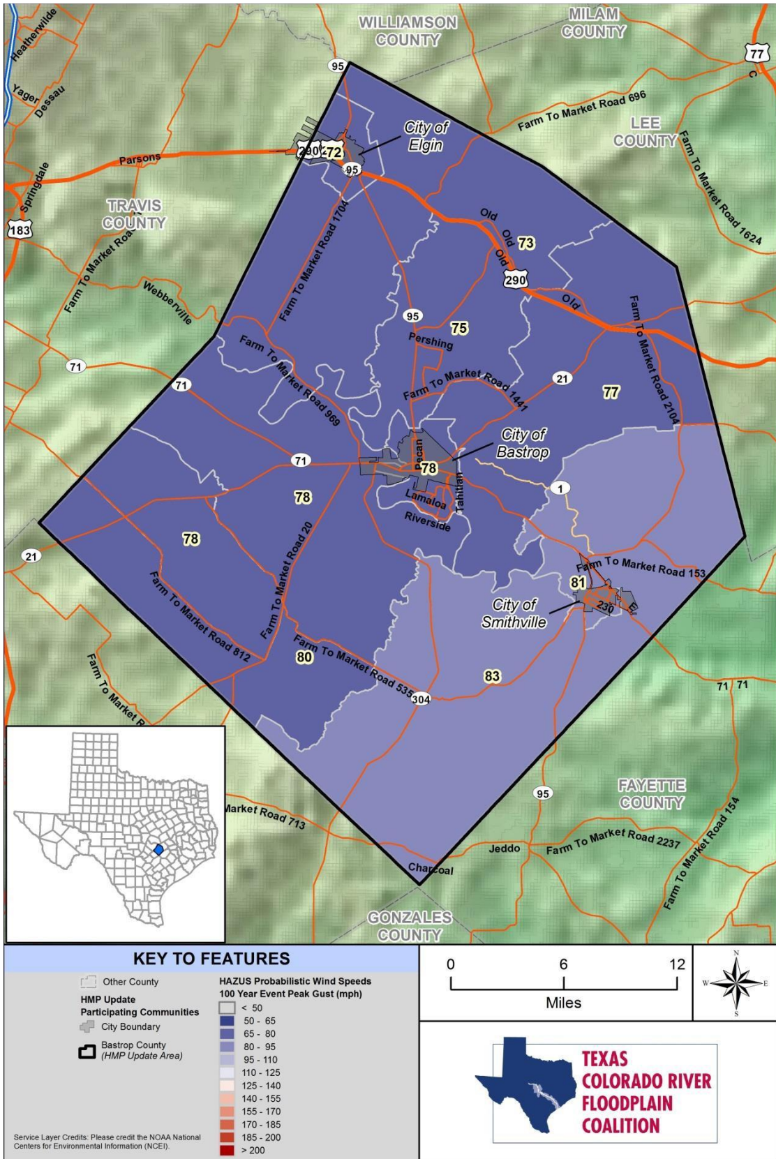
Figure 13-4. 100-Year Probabilistic Peak Wind Gusts for Bastrop County
