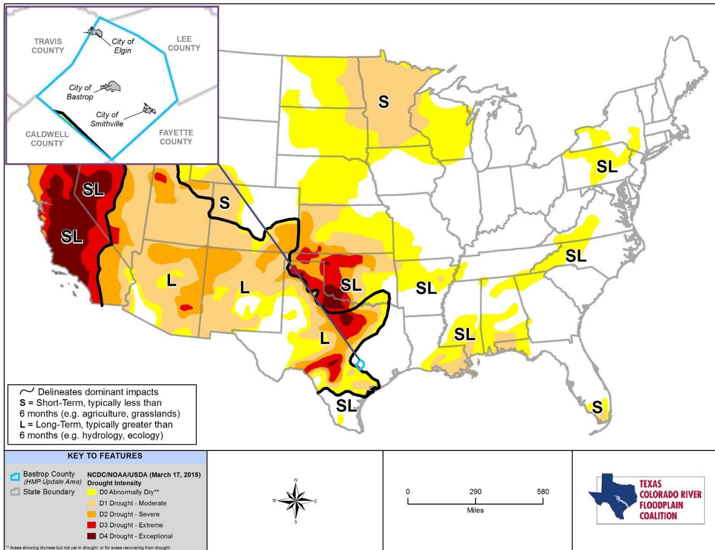
Figure 10-3. U.S. Drought Monitor, March 17, 2015
