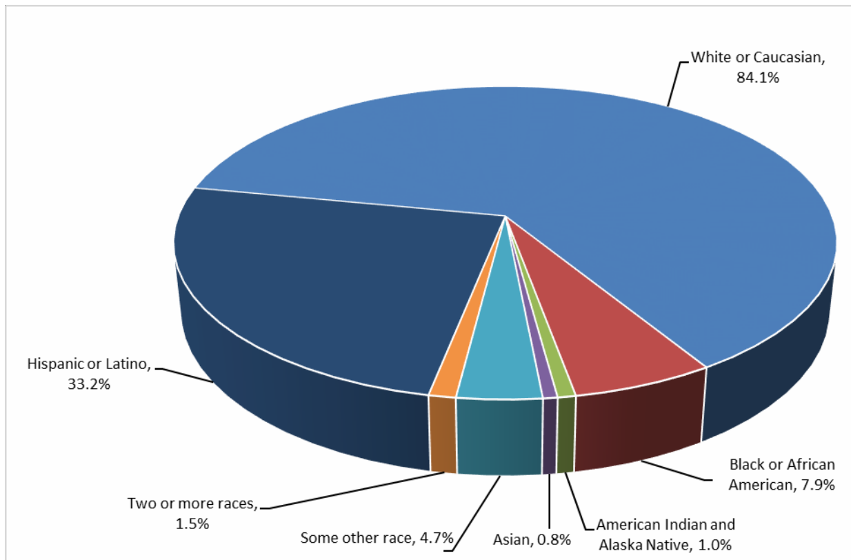
Figure 6-18. Bastrop County Ethnic Distribution
