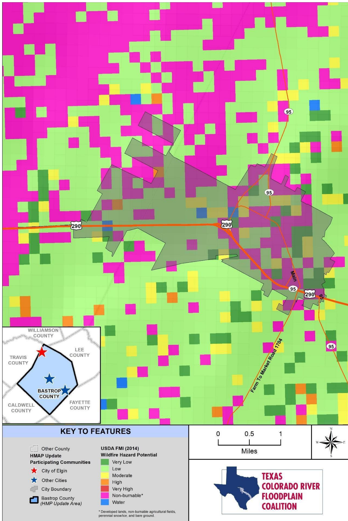
Figure 16-18. City of Elgin Wildfire Hazard Potential
